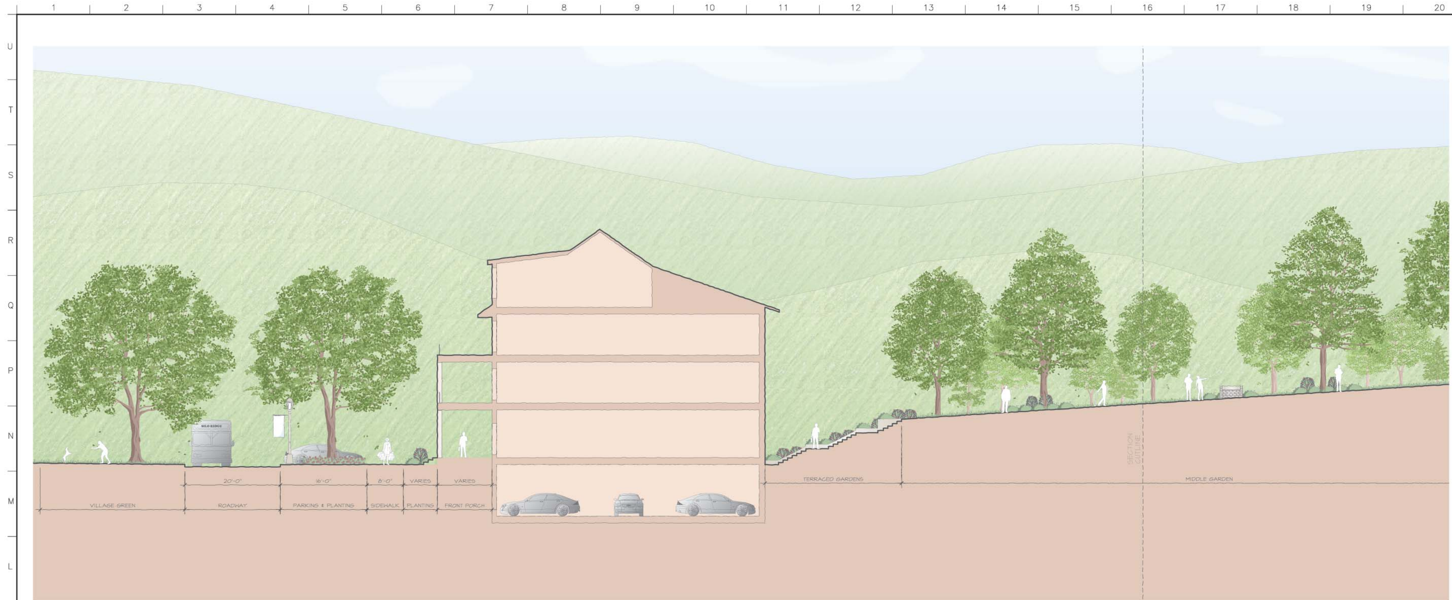
K1 SECTION THROUGH SHARED GARDENS SCALE: 1/8" = 1'-0"
