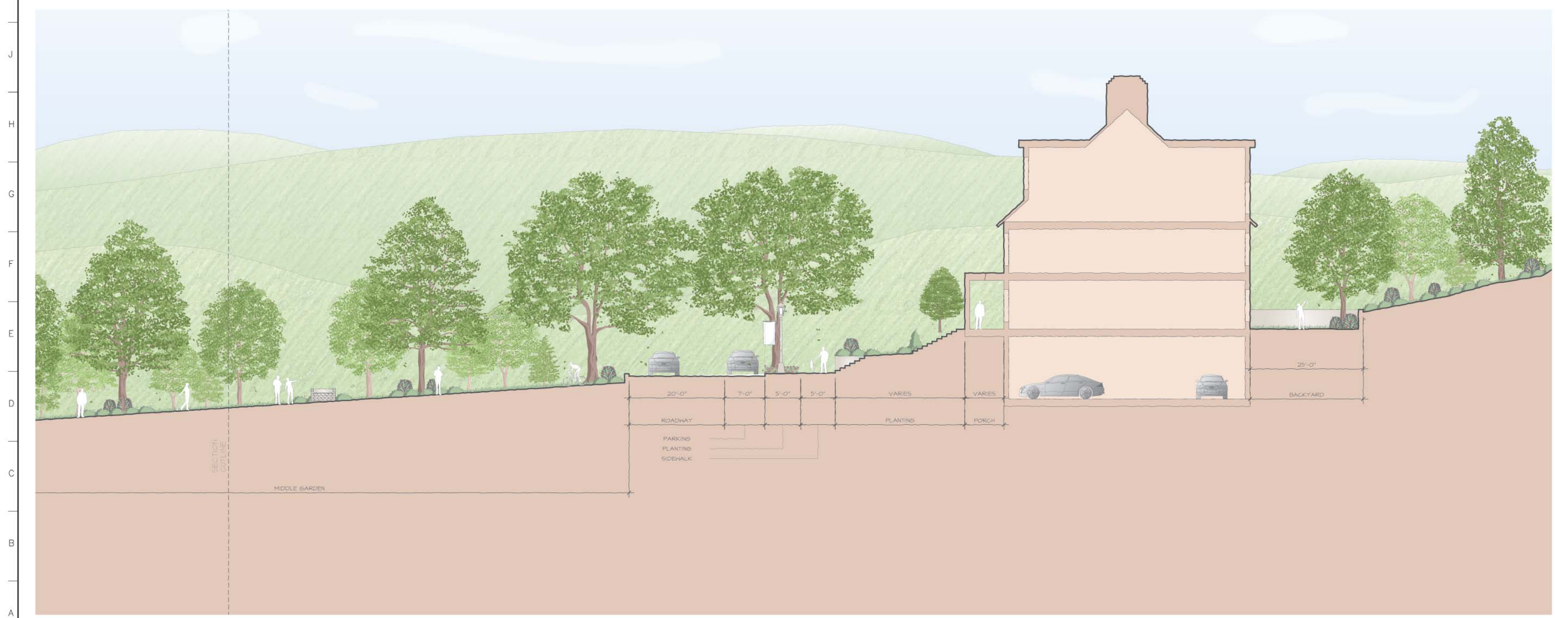
A1 SECTION THROUGH SHARED GARDENS SCALE: 1/8" = 1'-0"
