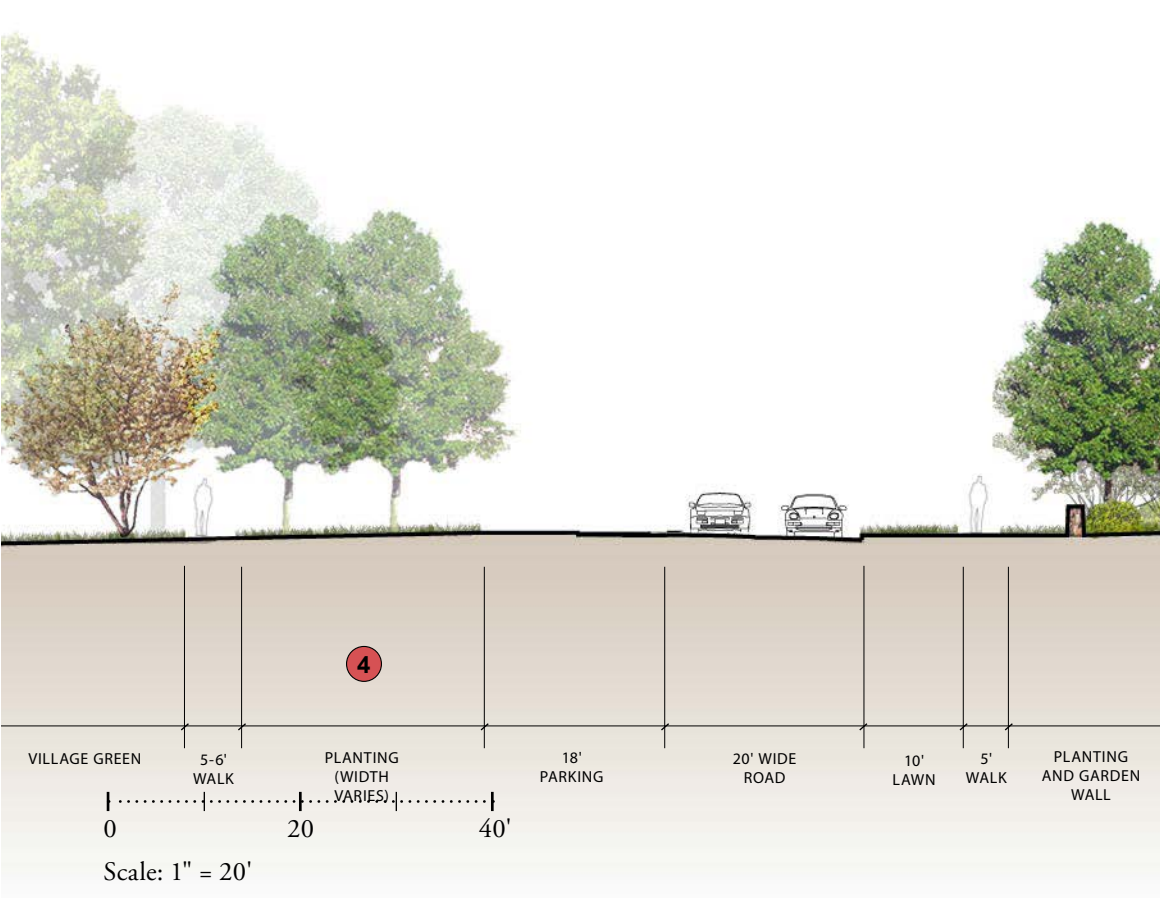
STREET SECTION 4: VILLAGE GREEN
