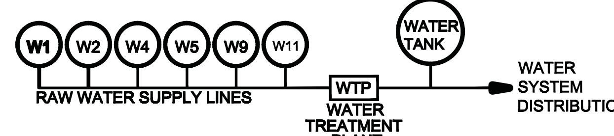
SCHEMATIC WATER SUPPLY SYSTEM DIAGRAM SPS-6 SCALE: NTS
